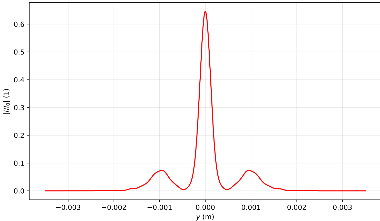
Intensity profile I(x = 0, y, z = 2.388)/I_0 , P_{in}=8.5P_{cr} , artificial time
